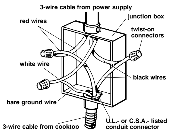
Grounded neutral Figure 2
