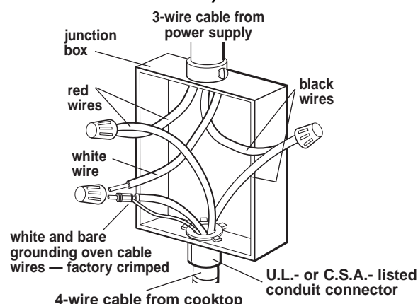
Grounded neutral Figure 4
